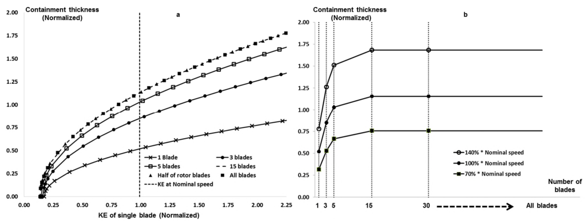
Figure 5. Containment analyses of simultaneous release of all blades and a sector of blades
