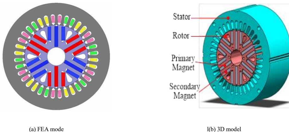
Fig. 1. The proposed machine configuration
