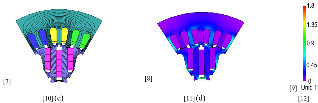
Fig. 5. field distributions when i_d=4.4A & i_q=0A , 0. (a) and (b) whole field (current and PM) and (c) and (d) armature field current (FP)
