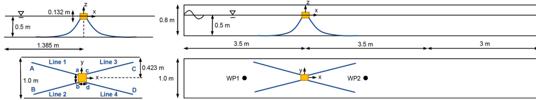
Fig. 7. The layout of the floating box with four catenary mooring lines in waves [24].
