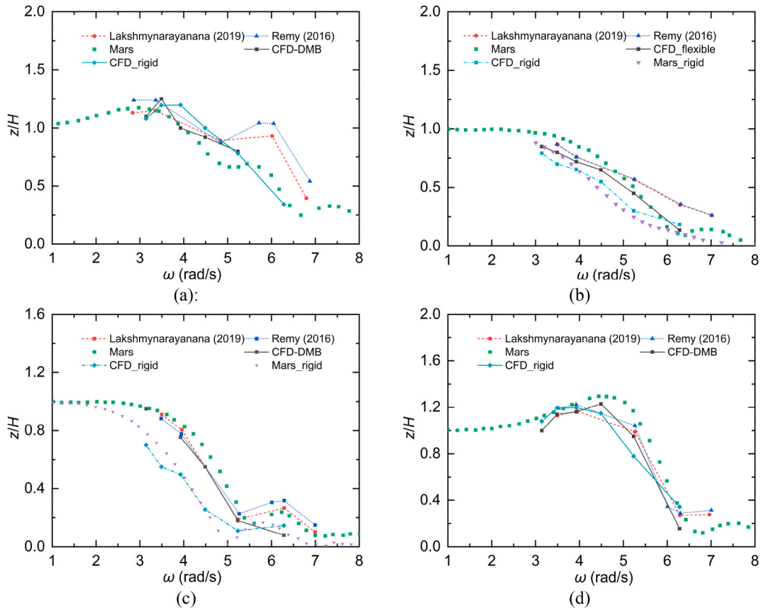
Fig. 11. Validation of heave displacements on VLFS sections in head waves: (a) Section #1 ( x/L = 0 ), (b) Section #5 ( x/L = 0.4 ), (c) Section #7 ( x/L = 0.5 ), (d) Section #12 ( x/L = 1 ).
