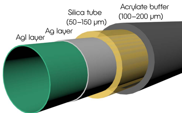
Fig. 1. Schematic showing the construction of a hollow silica waveguide. The values indicate the radial thicknesses of the silica and acrylate of the smallest (300 \mu\text{m} bore diameter) and largest (1000 \mu\text{m} bore diameter) commercially available waveguides from Polymicro Technologies [19].
