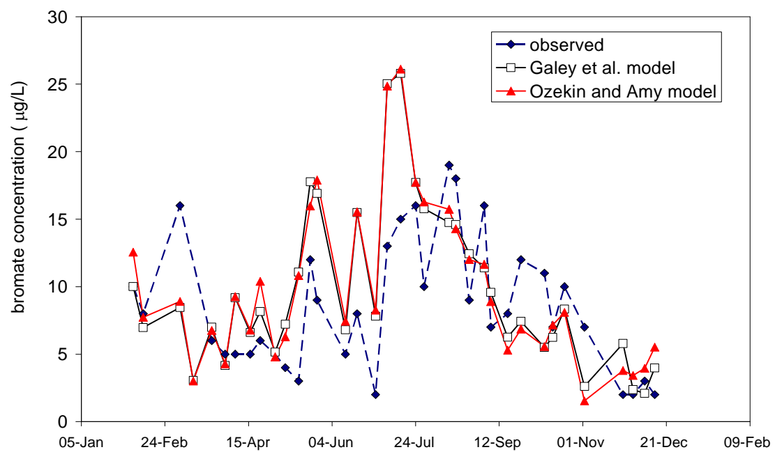
Figure 4. Observed bromate against predicted bromate using the models of Galey et al. (1997) and Ozekin and Amy (1997).
