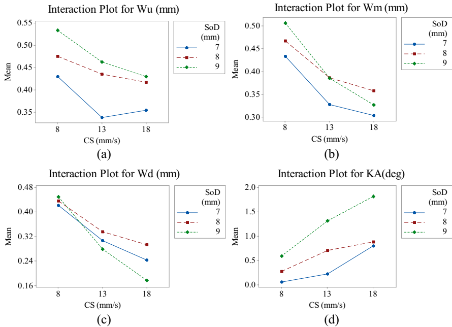
Fig. 5 Interaction plots between stand-off distance and cutting speed
