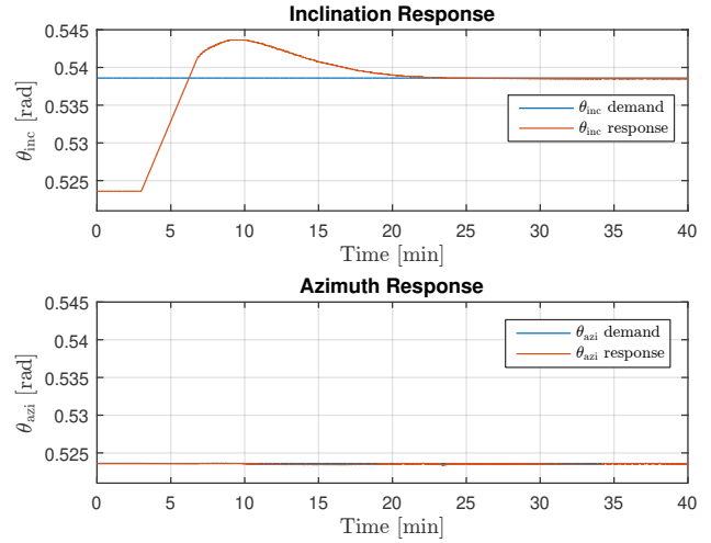
Fig. 9. Modified SP-BPI attitude response with azimuth response set at its initial angle of \pi/6 rad
