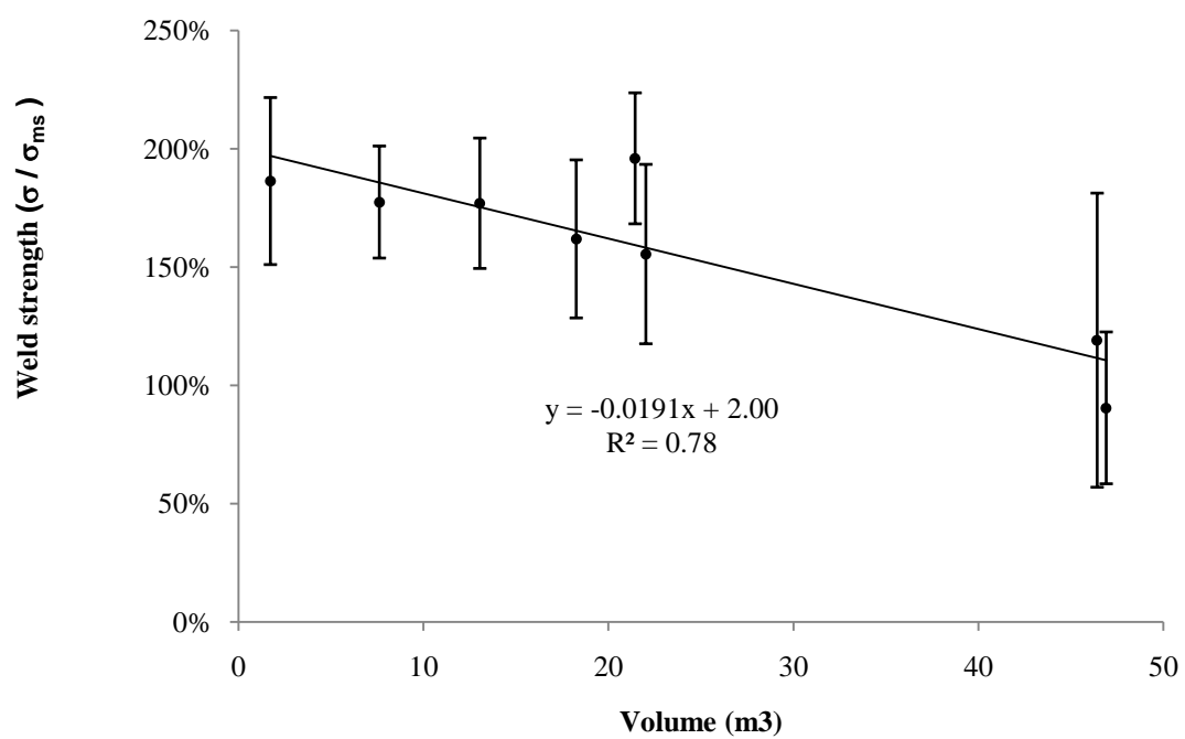
Weld strength vs. average permeate volume per panel per CIP
