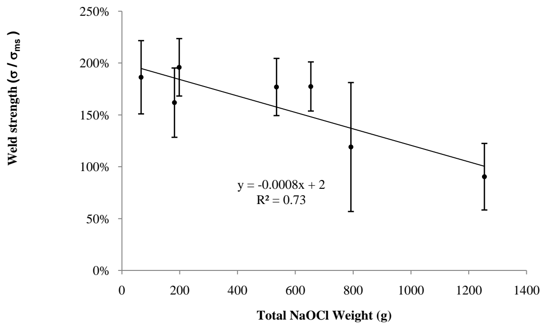
Total weight of NaOCl dosed over the life of the plant v.s. membrane welding strength
