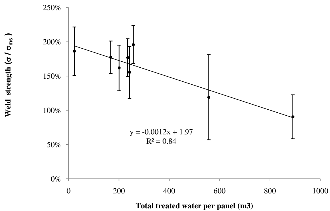
Total treated water per panel vs. membrane weld strength
