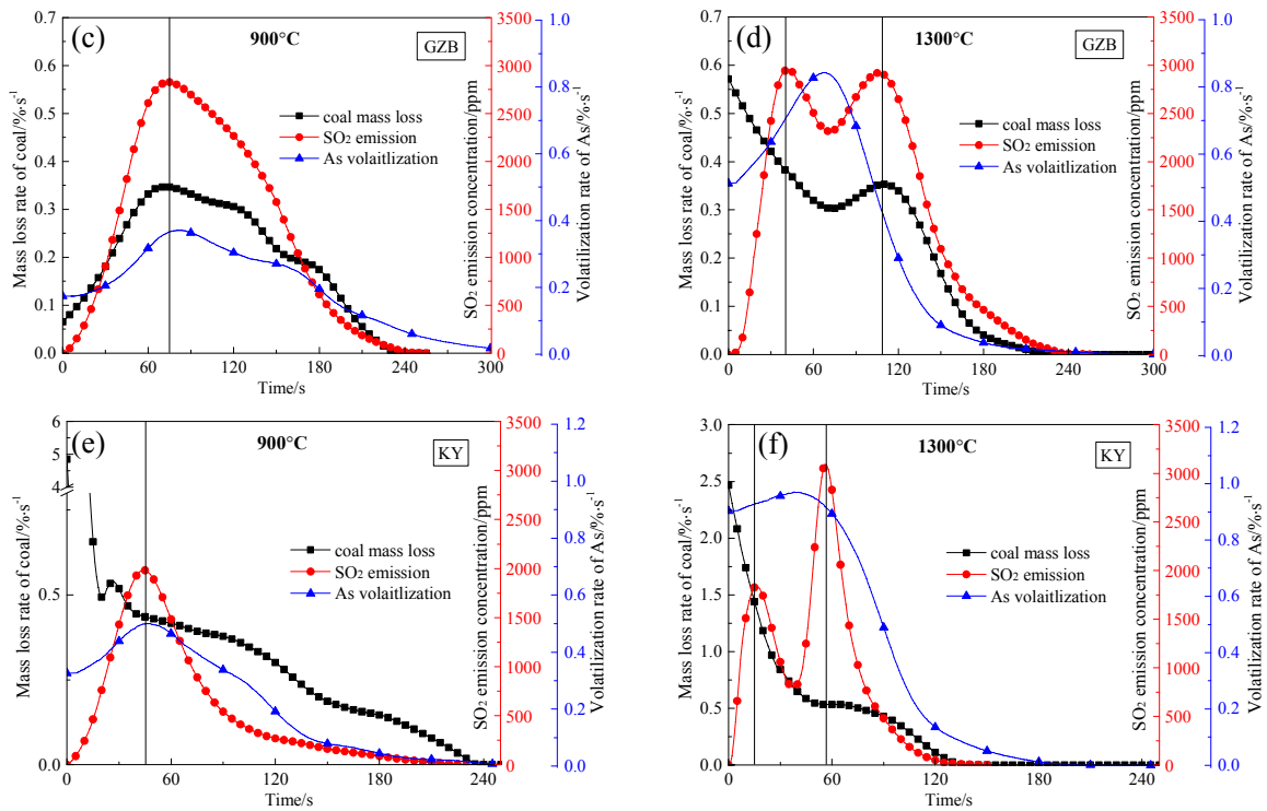
Figure 7: Simultaneous volatilization of arsenic and SO 2 during isothermal coal combustion [66] (a)GZA coal at 900°C; (b)GZA coal at 1300°C; (c)GZB coal at 900°C; (d) GZB coal at 1300°C; (e) KY coal at 900°C; (f)KY coal at 1300°C
