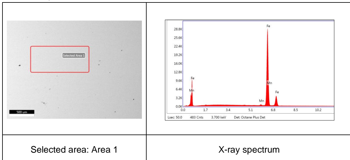
Figure E.5 Elemental analysis: 5.45mm main core, Area 1, 500μm
