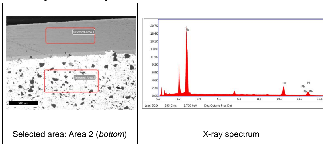
Figure E.6 Elemental analysis: 5.45mm core tip, Area 2, 500μm
