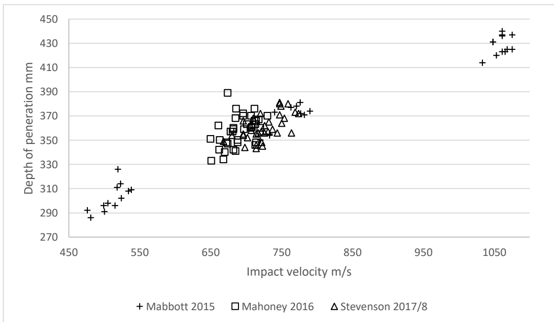
Figure 3.5 10% gelatine (4 °C) calibration data (Stevenson 2018 current study, compared to historical data [44,59]. Mabbott’s data included calibration using different velocities, hence the outlying clusters of data points seen on the graph)
