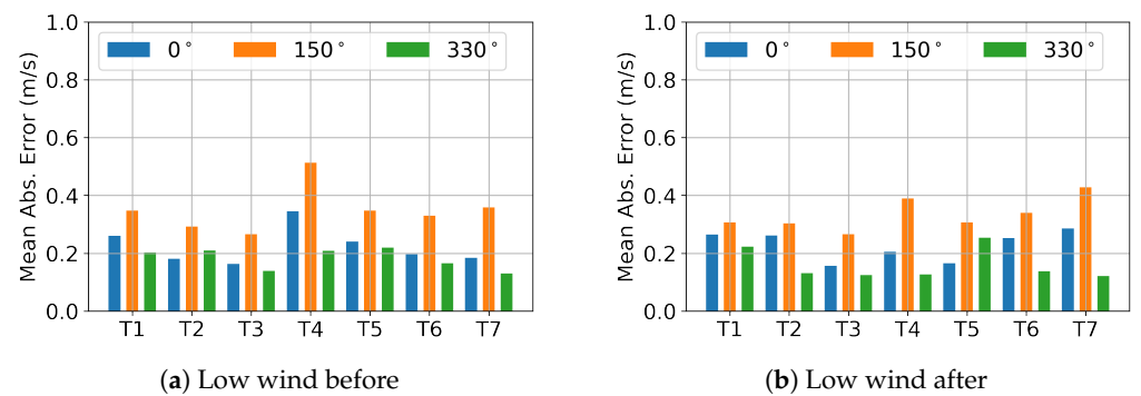
Figure 17. The mean absolute error between simulation and measurements for the sectors 0°, 150° and 330°, before and after the replacement of the T4 nacelle anemometer: low wind regime.
