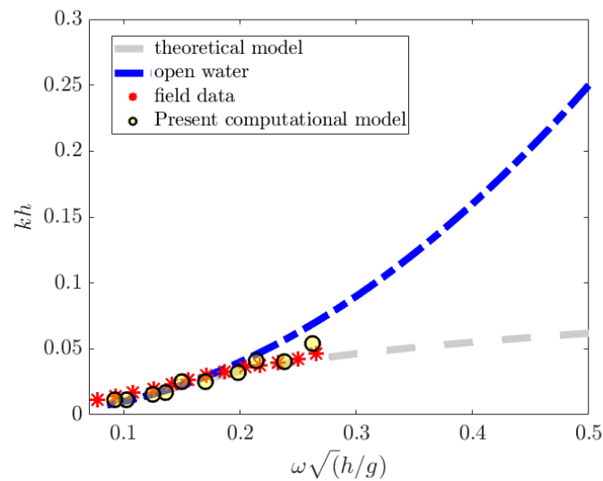
Figure 17. Dispersion curves of waves propagating in the covered (markers and dashed curve) and uncovered sea (dash-dotted blue curve). Field data (* markers) are taken from [33]. The dashed curves show the dispersion curve constructed using Equation (5). The results of the present model (circle markers) are found by running the model for small-scale ice.
