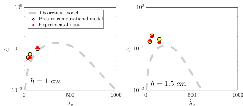
Figure 14. Comparison between decay rates given by the present computational model and the experimental values presented in Yiew et al. [53]. The dashed curves show the decay rate vs. open-water wavelength curves constructed by using Equation (5). Left and right panels respectively show the results corresponding to the ice covers with thicknesses of 1 and 1.5 cm.
