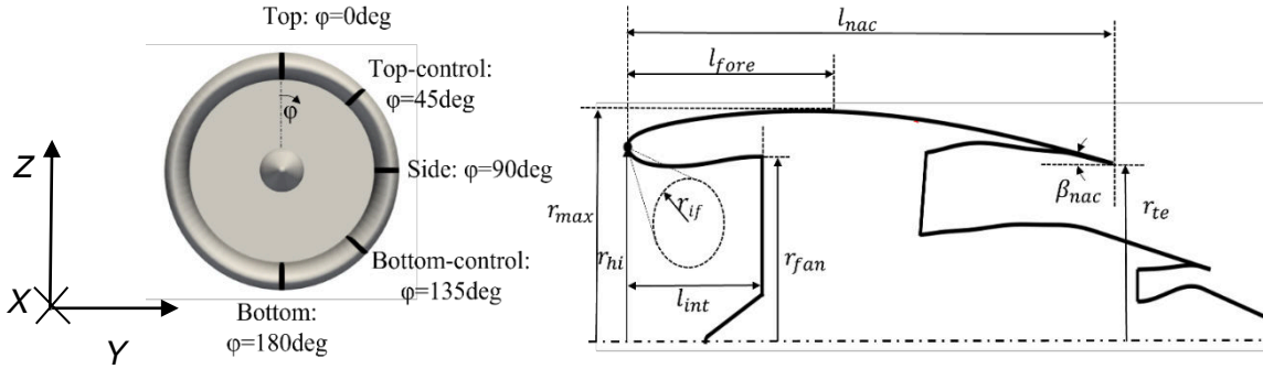
Figure 3 – Geometric parameterisation of the 5 aerolines (left) and the geometric parameters for each aeroline (right).
