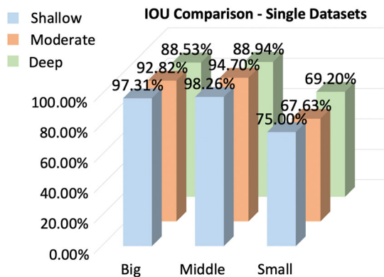
Fig. 8 Comparison of average intersection-over-union (IOU) of testing sets
