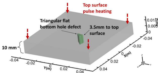
Fig. 4 Defective specimen model with a triangle shape flat bottom hole
