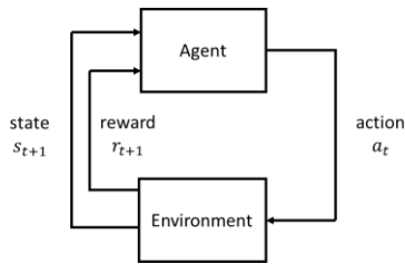
Fig. 2. RL Agent seeks to maximize cumulative reward obtained
