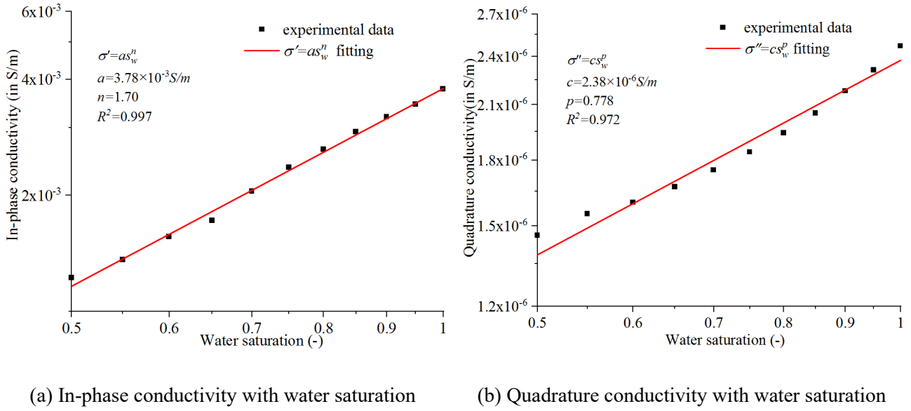
Fig. 5 Correlations between parameters of the complex conductivity at the peak frequency and water
