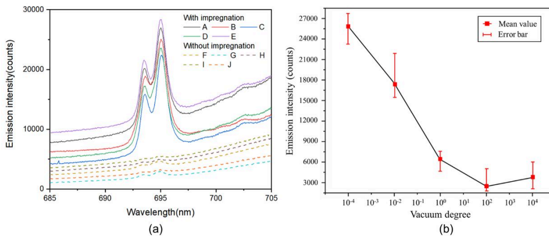
Fig. 4 (a) Comparison of the detected intensities of \text{Cr}^{3+} luminescence emitted by the TGO and passing through the YSZ TC, before and after the mineral-oil-impregnation treatment, at a vacuum degree of 10^{-4} . (b) Change in average intensities of \text{Cr}^{3+} luminescence as a function of vacuum degree.
