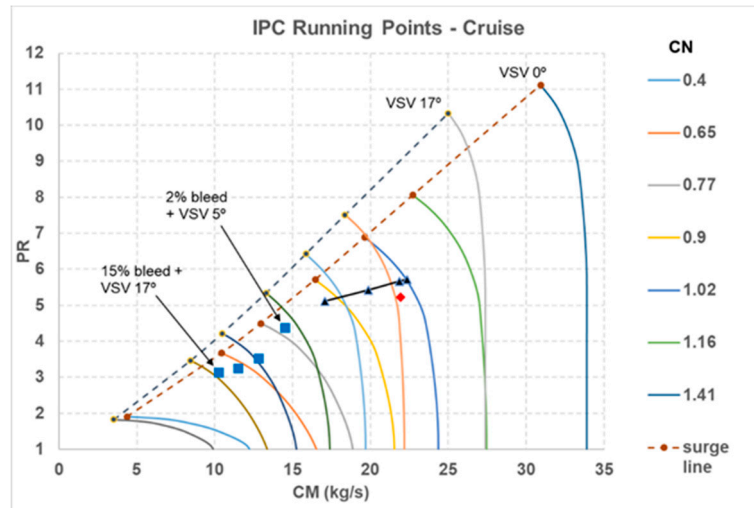
Figure 10. IPC running line at cruise.
