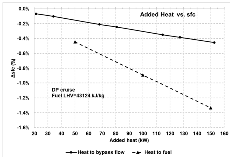
Figure 14. Added heat effect on SFC (DP study).
