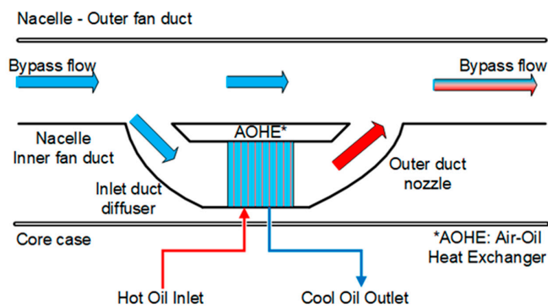
Figure 2. Bypass heat exchange system [32].
