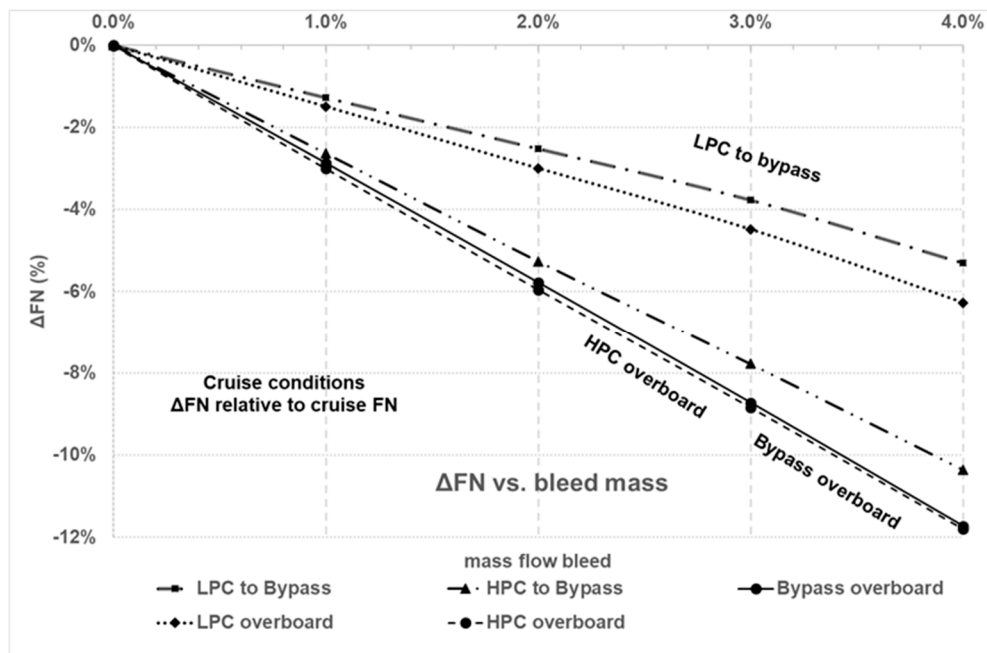
Figure 17. FN change vs. bleed mass.
