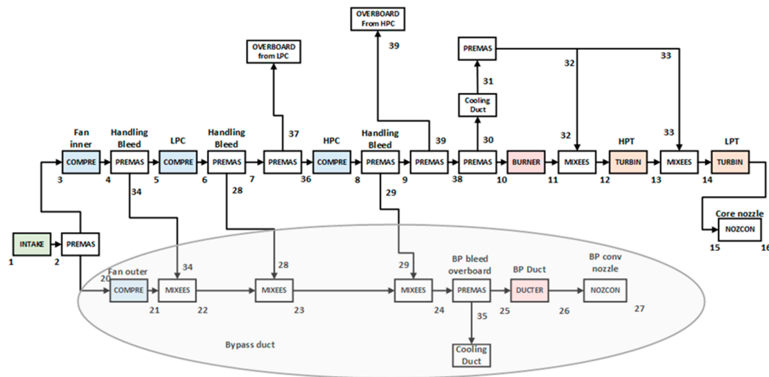
Figure A1. Engine model drawing (grey area: bypass duct).
