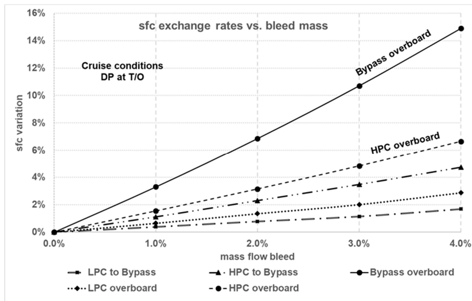
Figure 16. SFC exchange rates vs. bleed mass.
