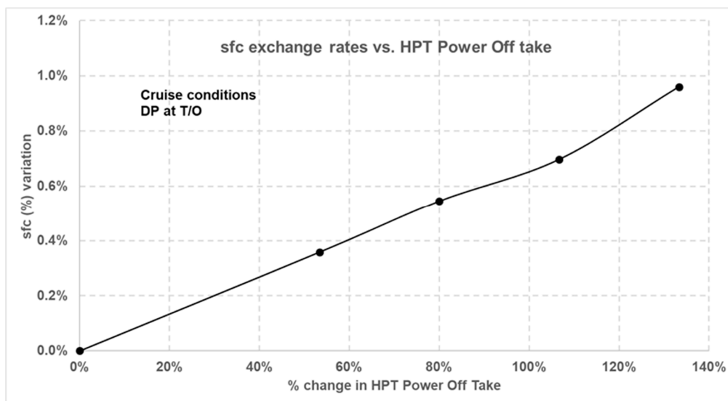
Figure 19. SFC exchange rates vs. HPT power offtake.
