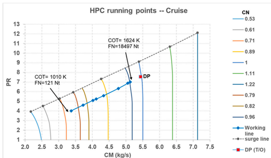
Figure 11. HPC running line at cruise.
