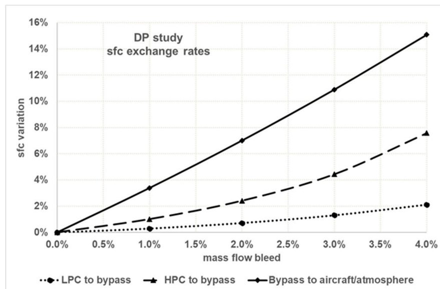
Figure 13. Bypass duct mass flow effect on SFC (DP study).
