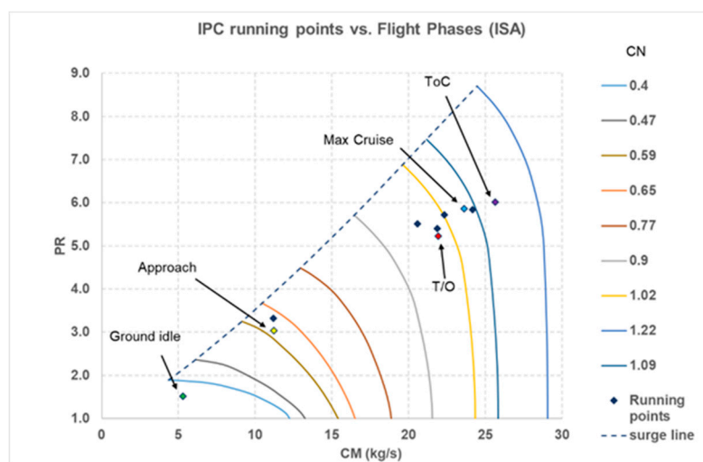
Figure 9. IPC running points at different flight phases (ISA).
