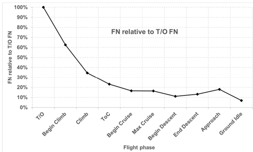
Figure 4. FN profile relative to T/O value.
