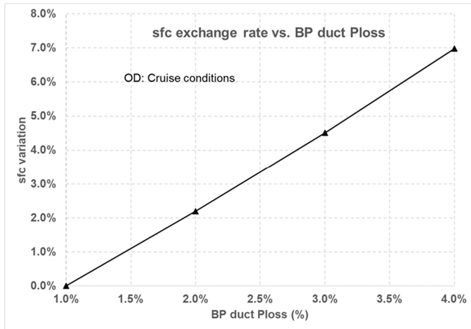
Figure 15. Effect of bypass duct pressure loss.
