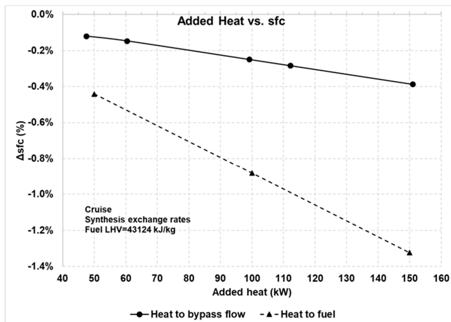
Figure 18. Added heat effect on SFC (synthesis exchange rates).
