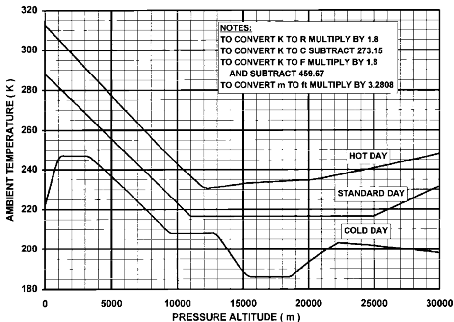
Figure 5. ISA hot and cold day ambient temperature variations with altitude [45].
