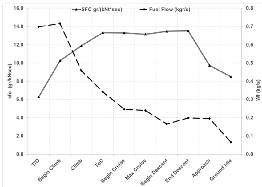
Figure 7. SFC and fuel flow at different flight phases.
