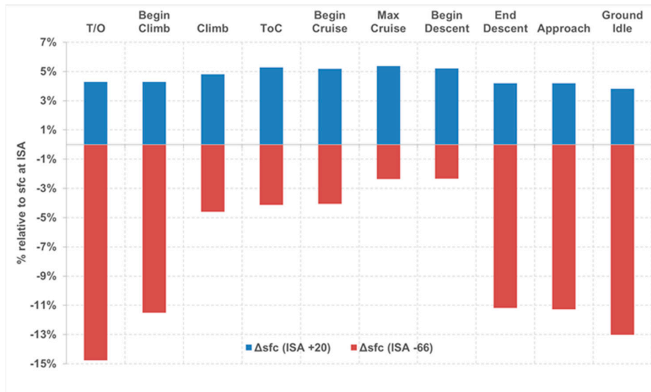
Figure 8. SFC variation due to ambient conditions.
