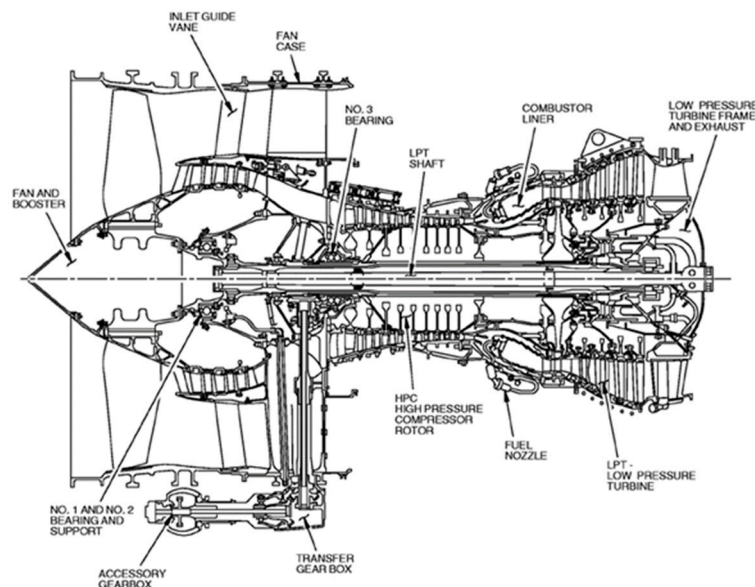
Figure 3. CFM56 drawing [33].
