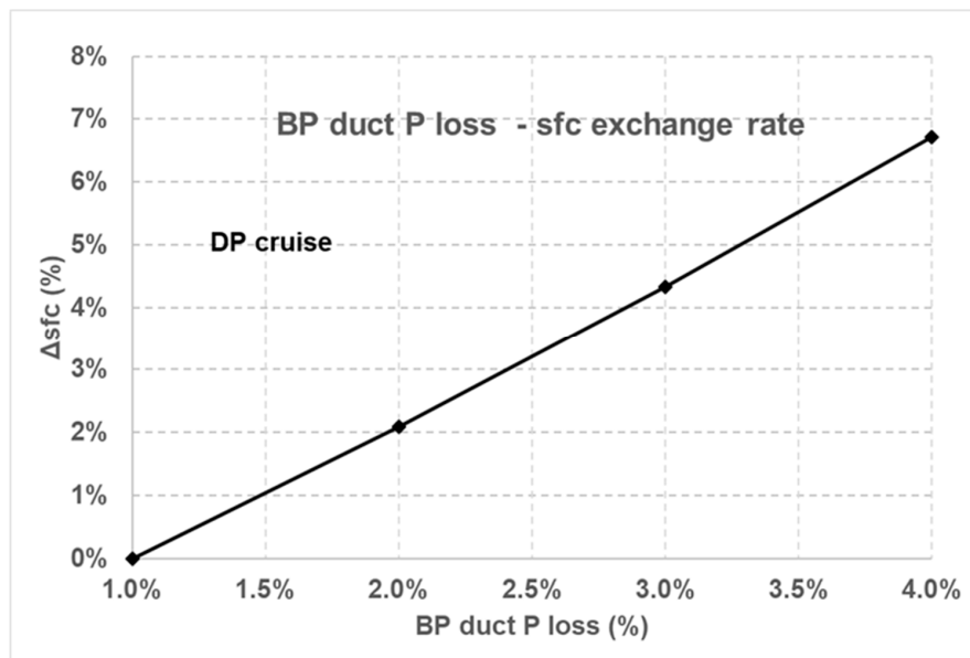
Figure 12. Bypass duct P loss effect on SFC (DP at cruise).
