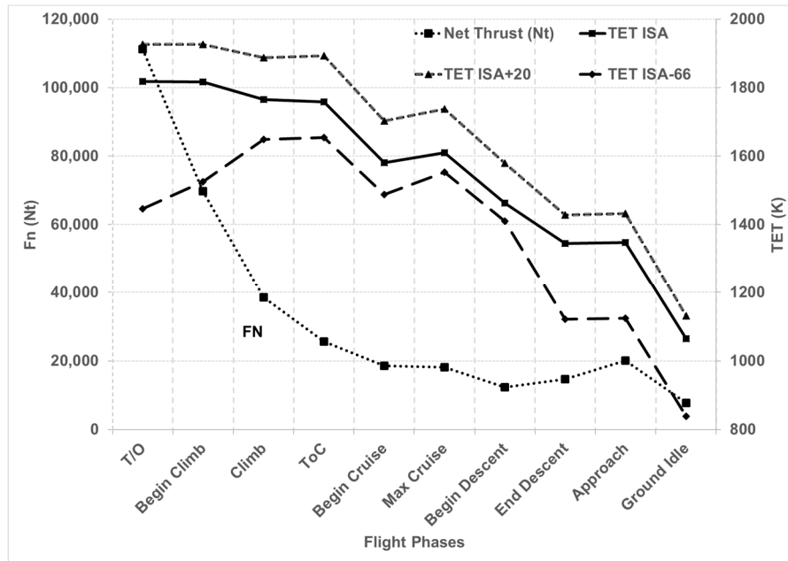
Figure 6. TET variation due to ISA ambient temperature variation.
