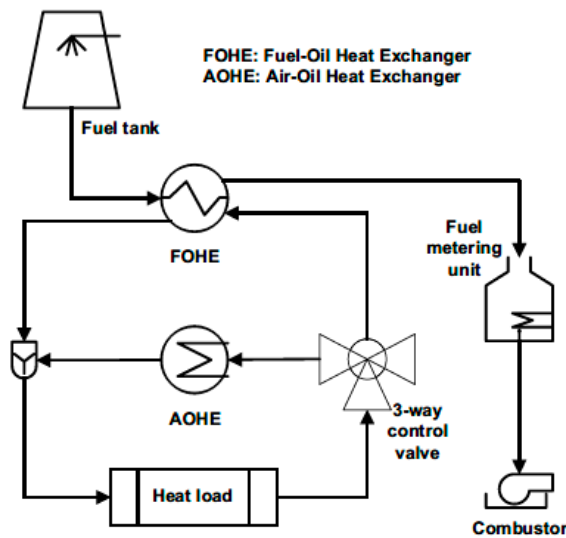
Figure 1. Typical thermal management system.
