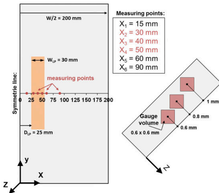
Figure 15 Schematic diagram of half of the CCT sample showing location of measurement points to define the residual stress field [22].
