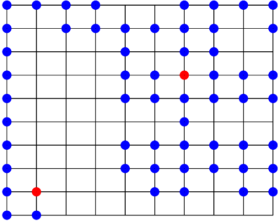
Fig. 4: An example showing that a solution space does not include optimal solution.
