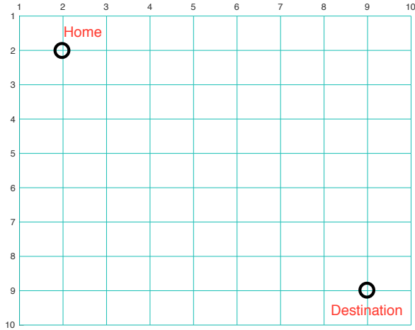
Fig. 2: An example of lattice graph representing the path model. The “home” is at (2,2) and the “destination” is at (9,9).
