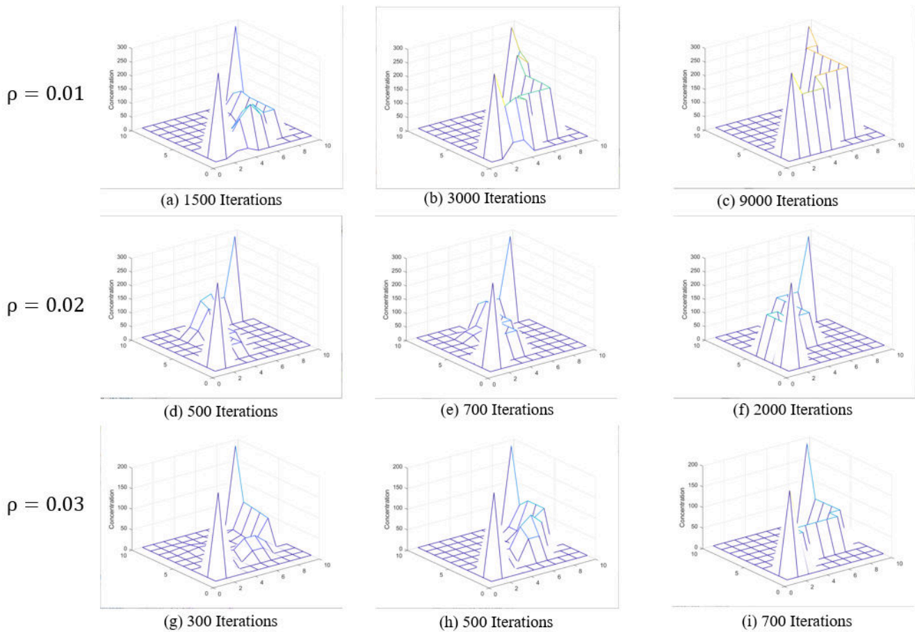
Fig. 5: Molecule concentration on lattice graph for different iterations and different degradation rates.
