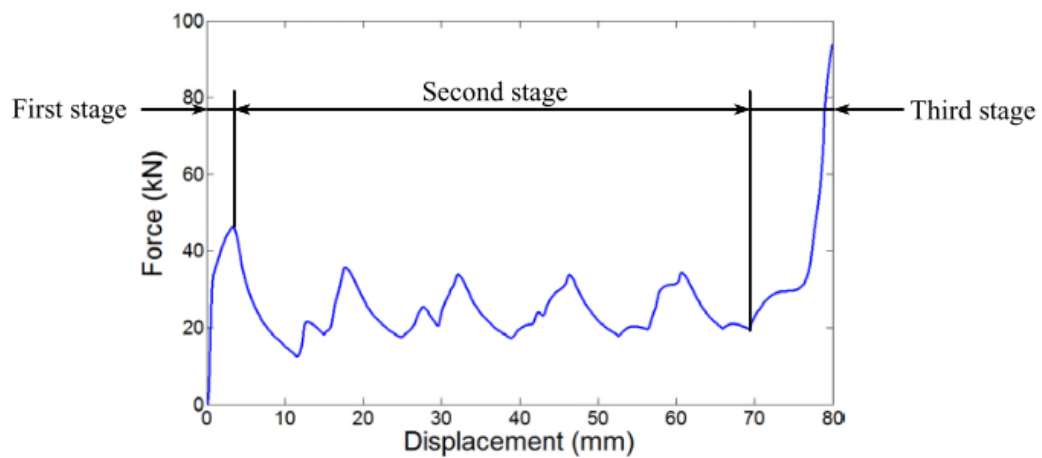
Figure 2 Typical load vs displacement curves of circular tubes in compression [8-9].
