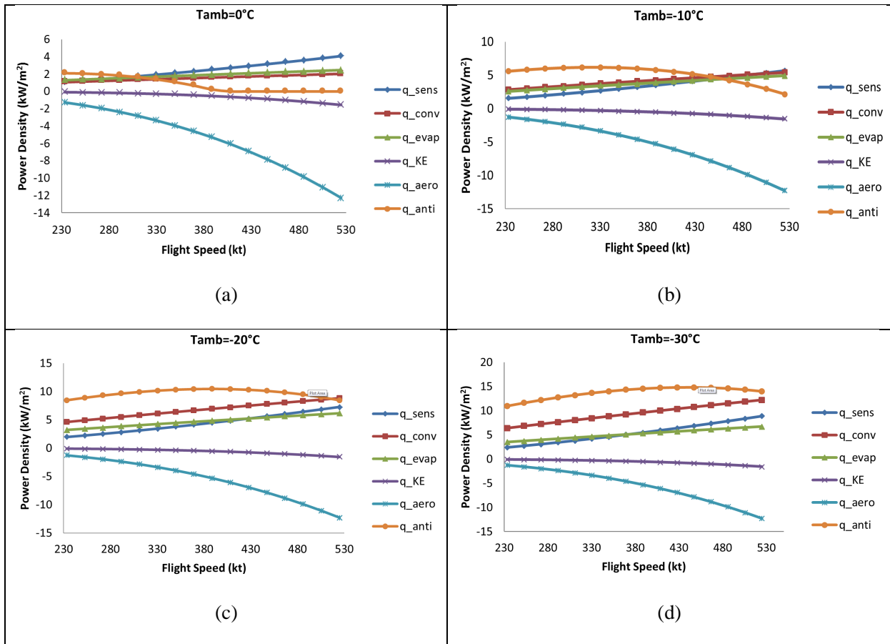
Fig. 15 Anti-icing Power Requirement at (a) 0 °C, (b) -10 °C, (c) -20 °C and (d) -30 °C
