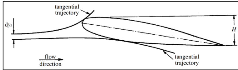
Fig. 8 Definition of Overall Collection Efficiency and Projected Height [11]
