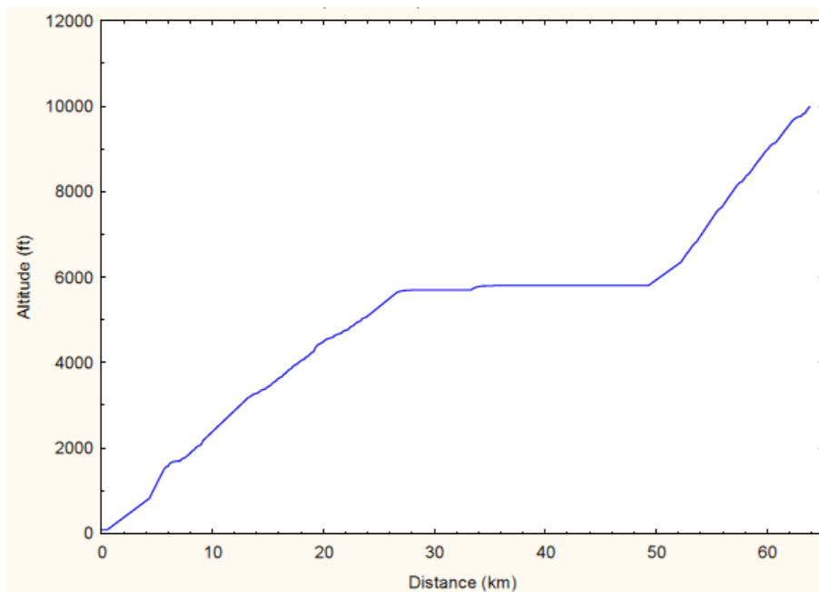
Fig. 21 A Tracked Departure from London Airport Heathrow to Amsterdam Airport Schiphol
