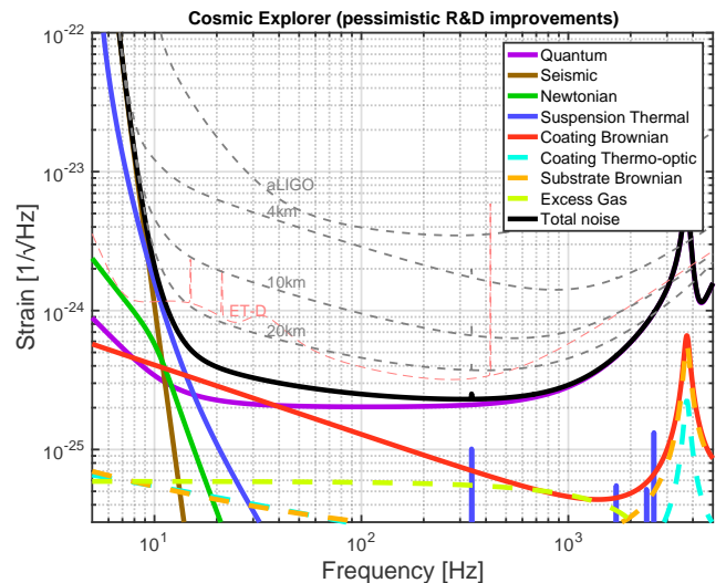
FIG. 3. Similar to figure 2 but with coating and suspension thermal noise models which assume minimal progress. The wide-band signal extraction choice is made to minimize the impact of CTN. The proximity of the dashed grey 4 km curve to the Advanced LIGO reference curve reflects the fact that coating technology, which is nearly limiting in Advanced LIGO, becomes dominant over a range of frequencies given the reduction of quantum noise assumed for the future.
