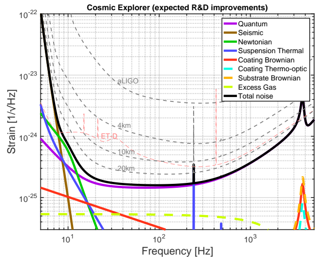
FIG. 1. Target sensitivity for a next generation gravitational-wave detector, known as “Cosmic Explorer” for its ability to receive signals from cosmological distances. The solid curves are for a 40 km long detector, while the dashed grey curves show the sensitivity of shorter, but technologically similar detectors; lengths are 4, 10 and 20 km. The Advanced LIGO and Einstein Telescope design sensitivities are also shown for reference.
