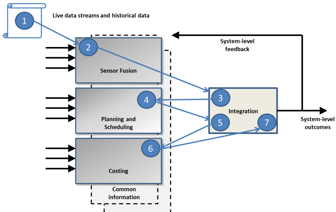
Figure 3: Schematic diagram of the AUTONOM Prototype
