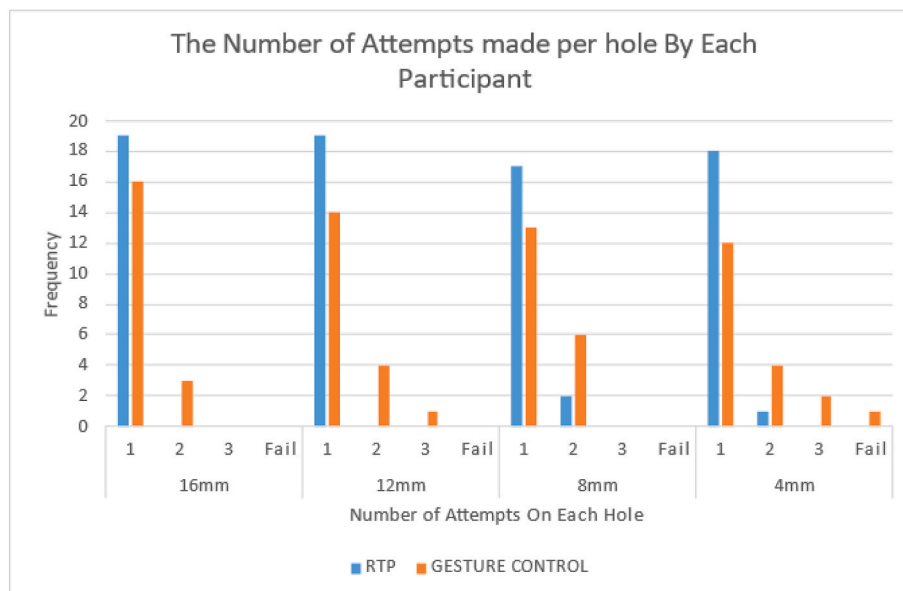
Fig. 12. A chart showing the frequencies of the number of attempts per hole across all participants.
