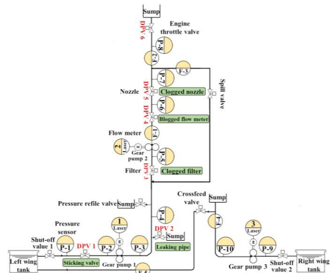
Fig. 1. The layout of the fuel rig system
