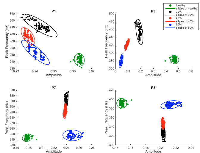
Fig. 5. The result of fault identification using the 95% confidence ellipse.
