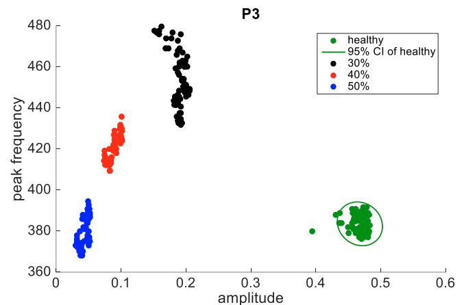
Fig. 3. An example of fault detection based on the channels P3, where the eclipse represents the 95% confidence level of healthy behaviour.
