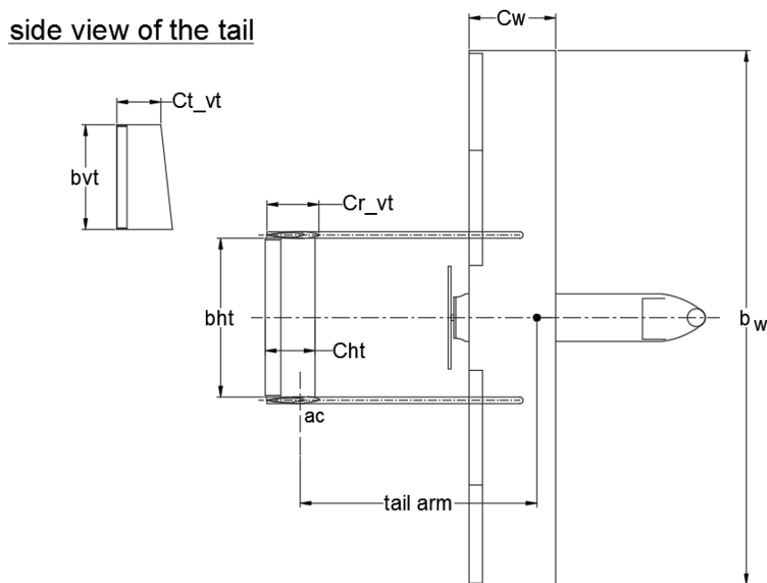
Figure 7. Definition of design variables for Aegis UAV with the U-tail shape.
