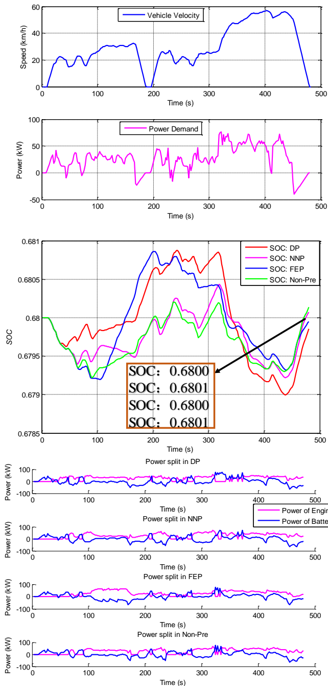
Fig. 7. SOC trajectories and power split for a simulation cycle with different control strategies.
