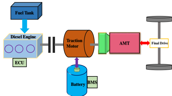
Fig. 1. Configuration of the parallel HEV powertrain.
