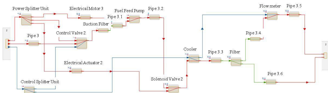
Fig. 6. Feed unit functional model
