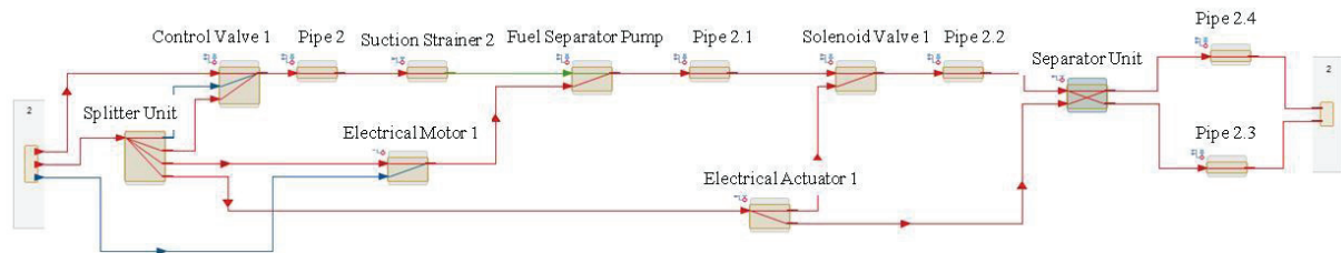
Fig. 5. MADe Separation unit functional model
