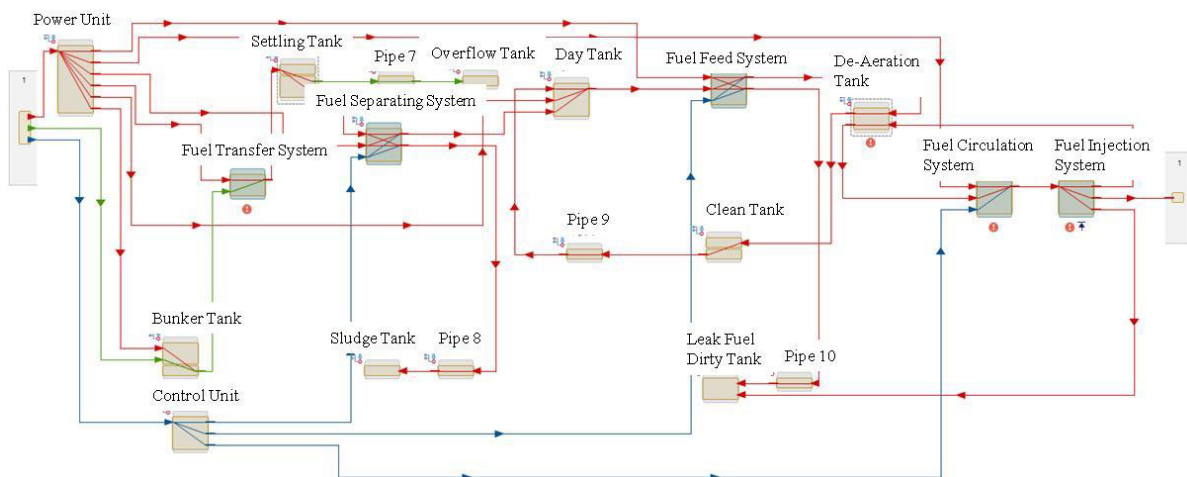
Fig. 4. MADe Fuel system functional model
