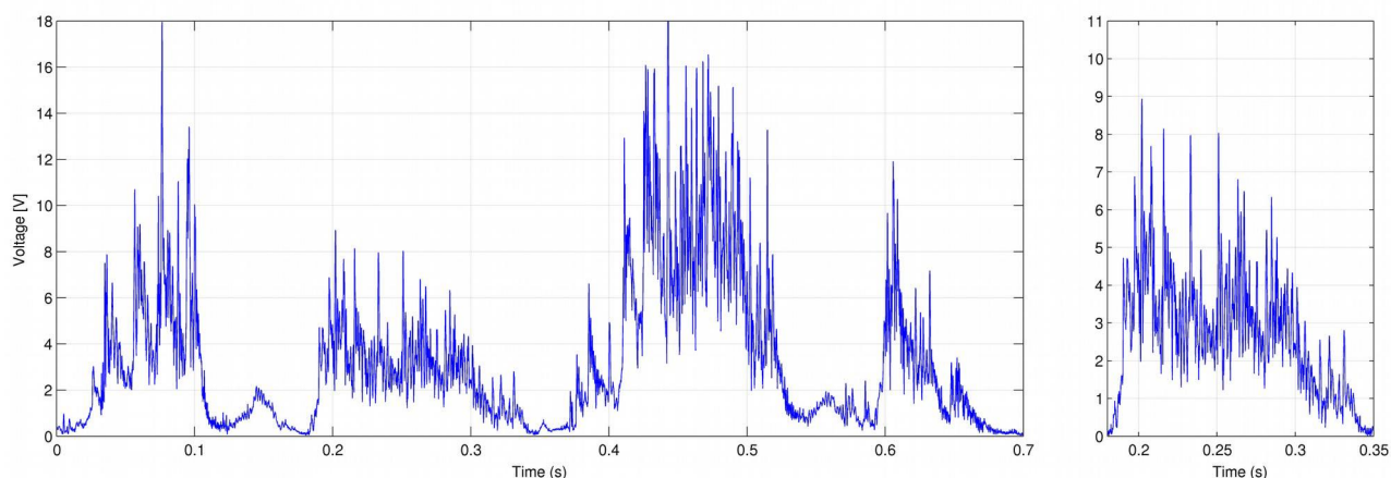
Figure 5: Voltage across load resistor (21.5 kΩ) for a run gait with 78 pletra. The detail on the right shows a more continuous generation (as compared to Figure 4)
