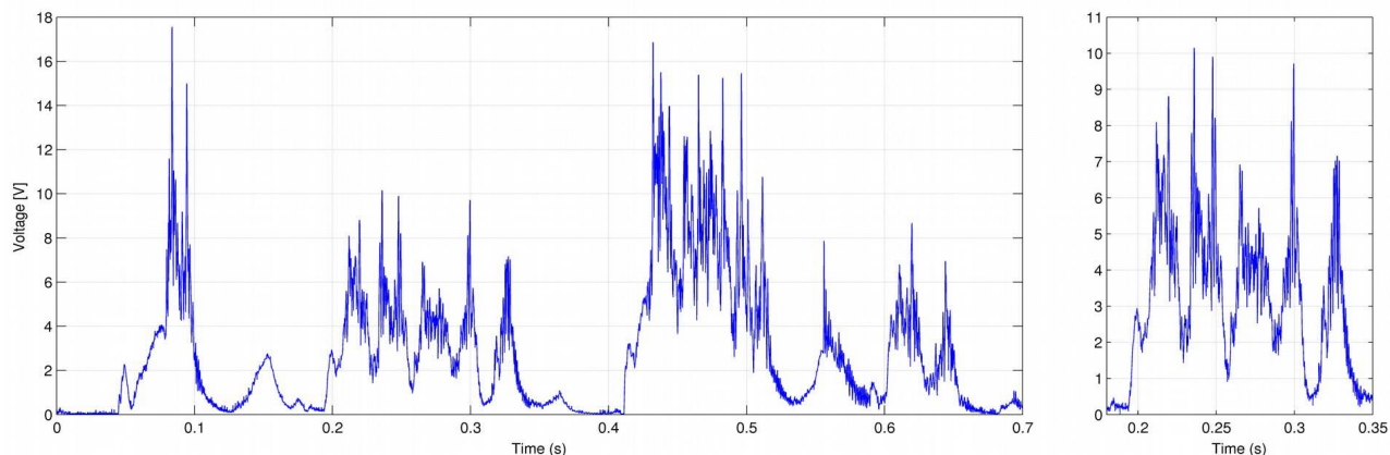
Figure 4: Voltage across load resistor (21.5 kΩ) for a run gait with 80 pletra. The detail on the right shows bursts of generation.
