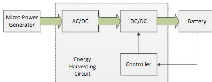
Fig. 1. Typical energy harvesting system diagram [4].
