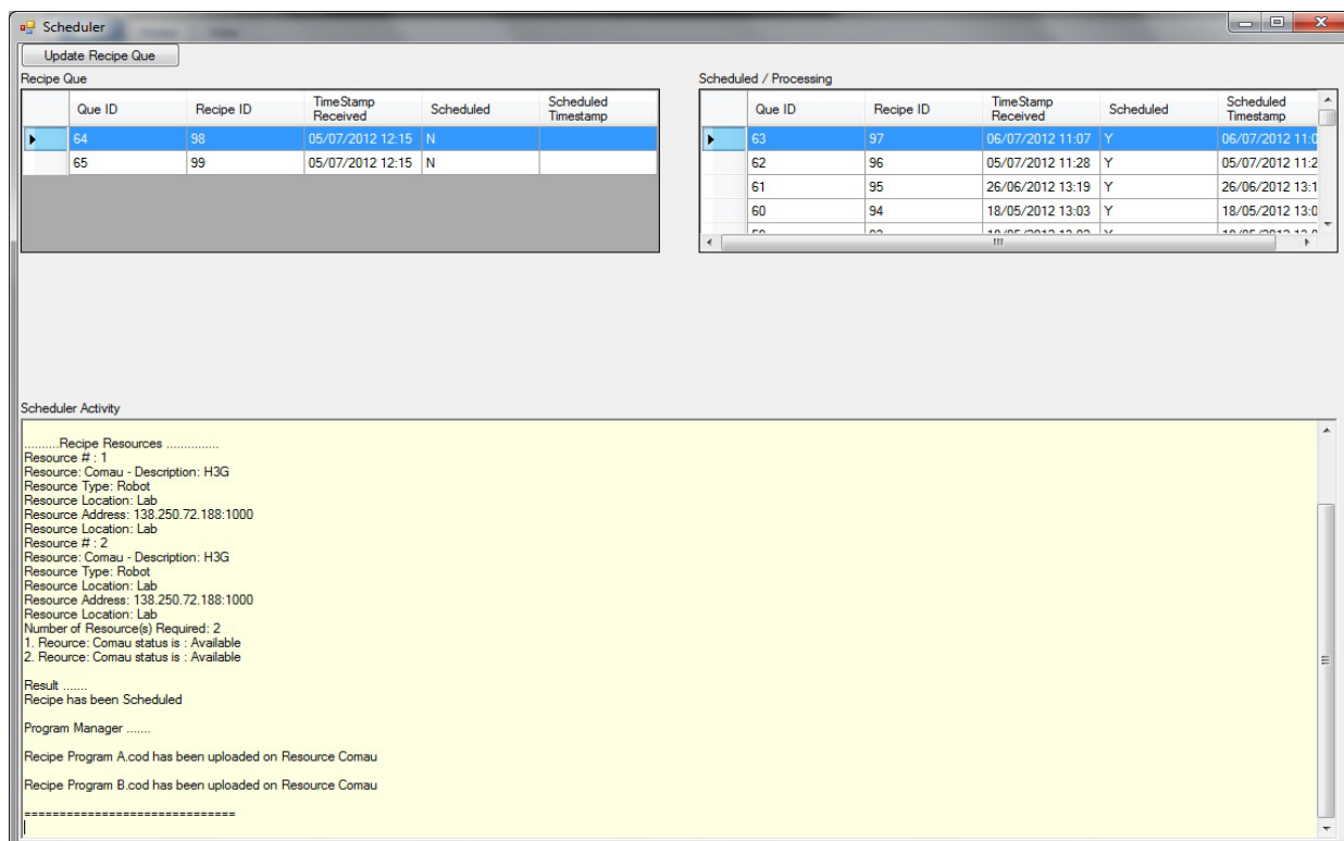
Figure 4: Scheduler interface.
