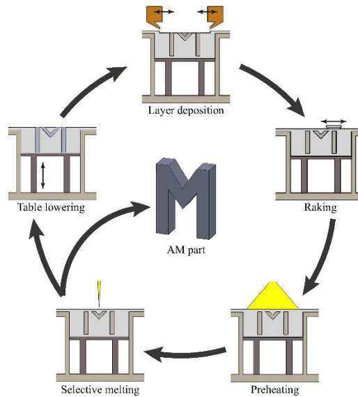
Figure 5. A schematic of the EBM process [53]
