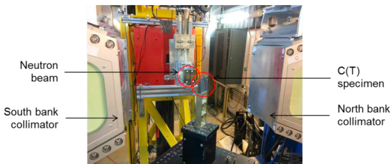
Fig. 3. Neutron diffraction experimental set up on Engin-X
