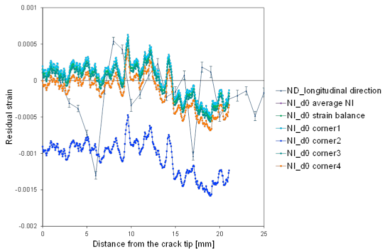
Fig. 6. Residual strains within the HAZ using neutron diffraction and neutron imaging techniques with different d_0
