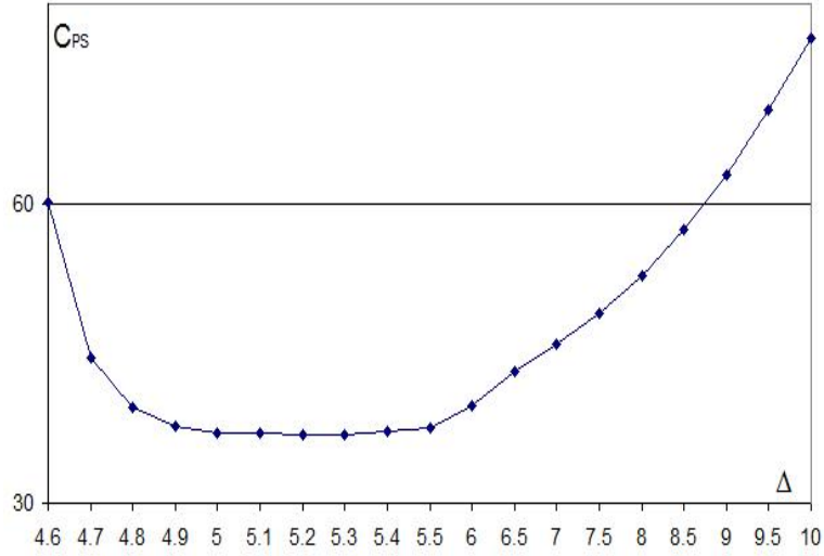
Fig. 2. Impact of PM quality on the expected long-run cost rate.
