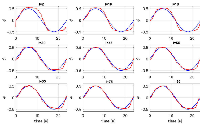
Fig. 5. The PI controller on trajectory I for during variation of \phi .
