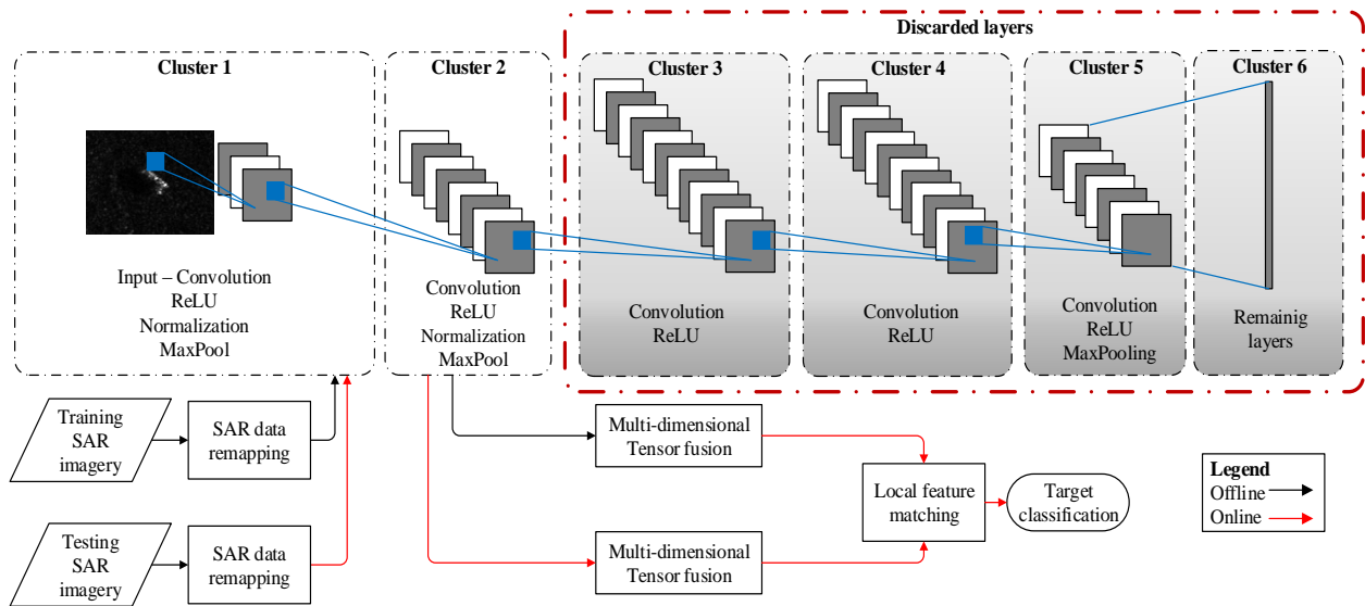
Fig.1 Proposed SAR ATR architecture showing activated cluster 2
