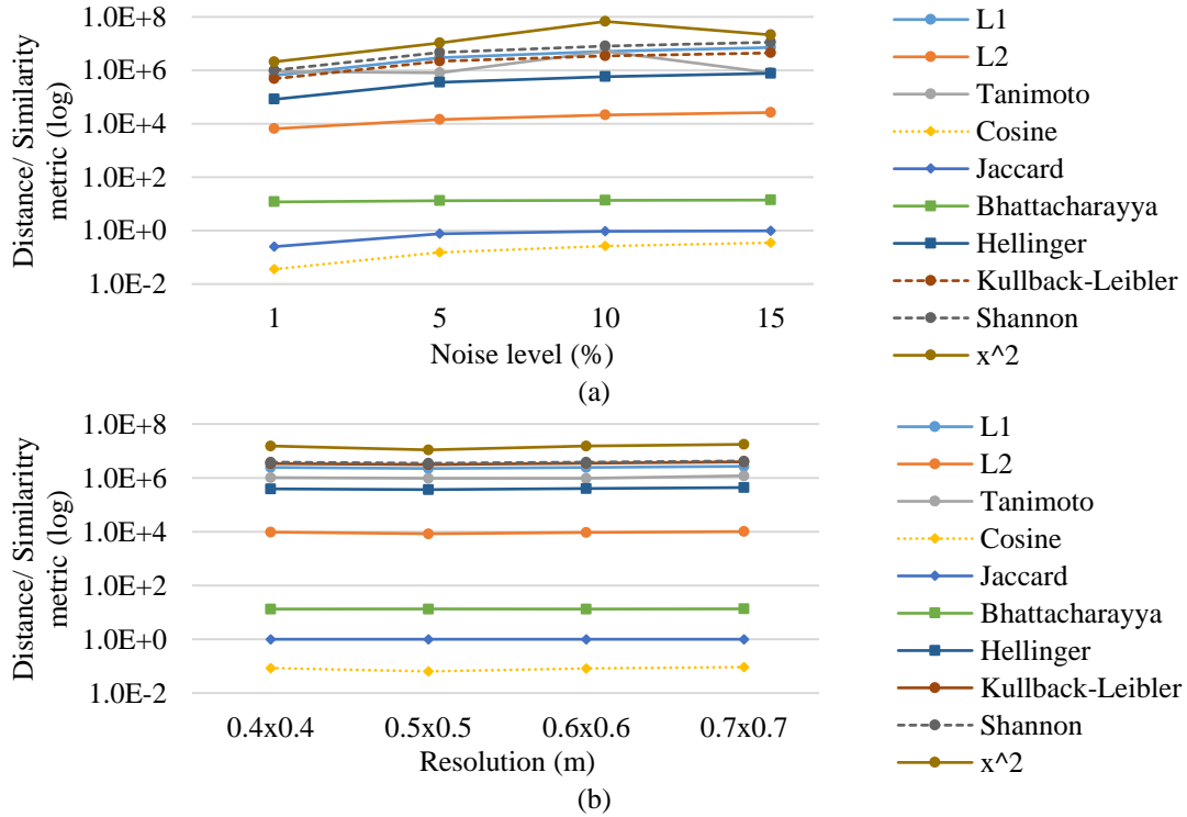
Fig. 9 Robustness in various nuisances and levels (a) noise (b) resolution
