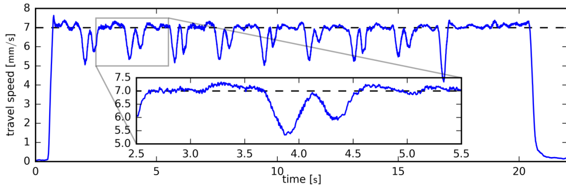
Figure 10 Travel speed profile for 10 mm o.width
