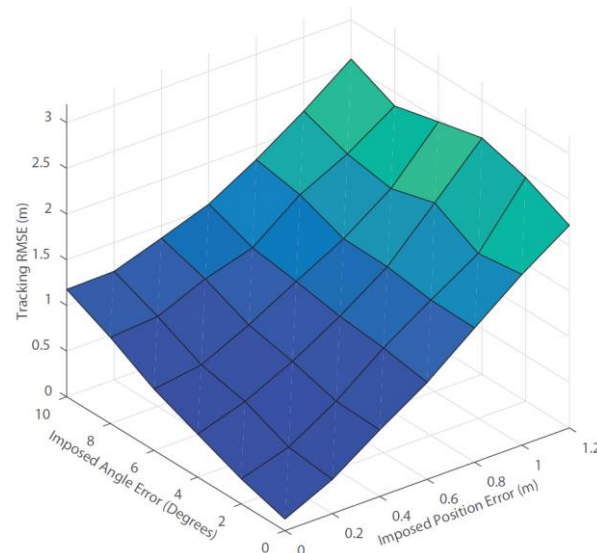
Figure 14. Tracking RMSE using a collaborative positioning algorithm. The corresponding tracking is significantly reduced by up to 50%.
