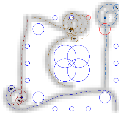
Figure 18. Monitoring mission—faulty scenario 2 (faulty sensors in red).
