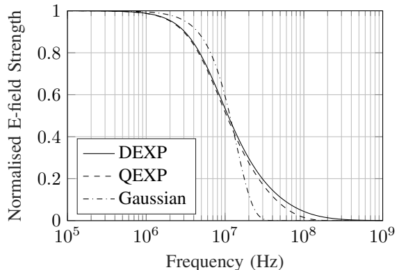
Fig. 6. Frequency response through lossless material.
