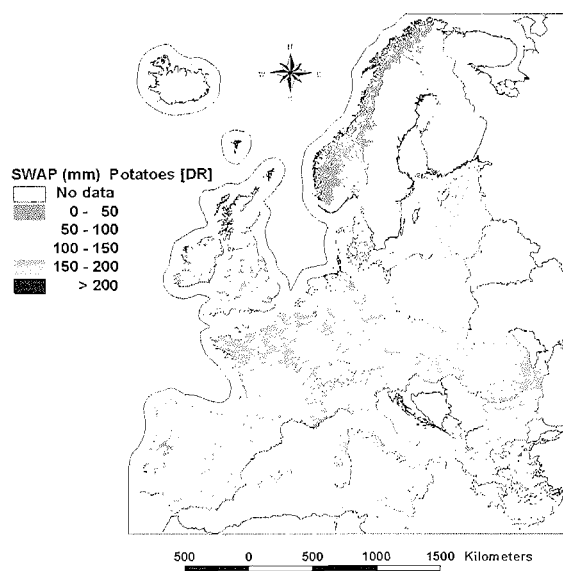
Figure 5. Soil water available to plants, SWAP (mm) for a short rooting crop e.g. potatoes.
