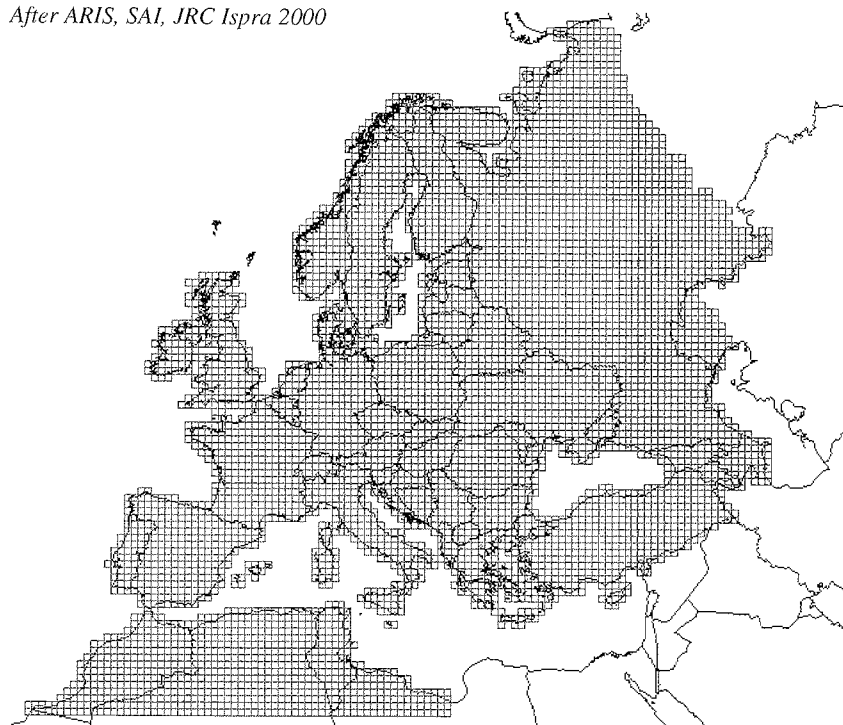
Figure 6. The 50 km × 50 km grid of the MARS meteorological database.
