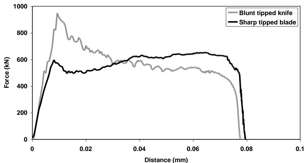
Figure 2. The force vs. displacement plots for blunt and sharp knives on 5.5mm thickness aramid-thermoplastic composite.
