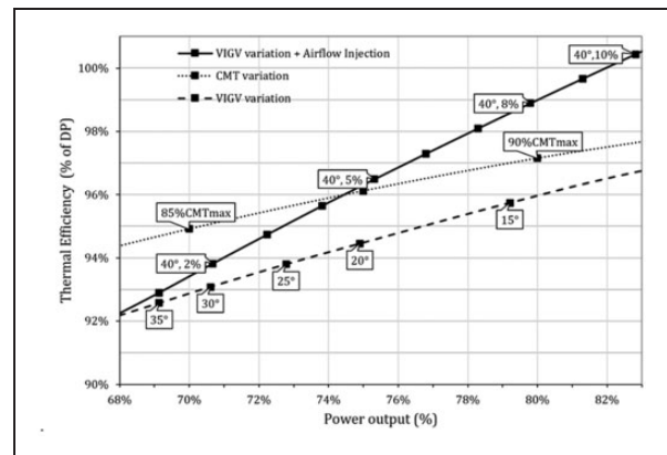
Figure 8. Thermal efficiency versus PO – with air injection and without (fixed and varied VIGV), CMT: combustor mean temperature; VIGV: variable inlet guide vane.
