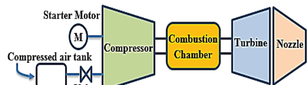
Figure 1 Schematic representation of the micro jet engine with air plus electric starting
