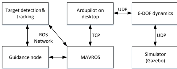
Fig. 4. The software in the loop test for the Pixhawk
