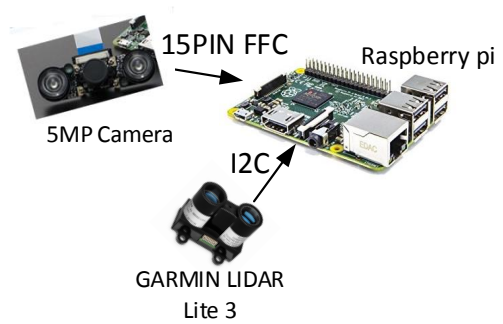
Fig. 2. The Sensor integration on the Raspberry Pi
