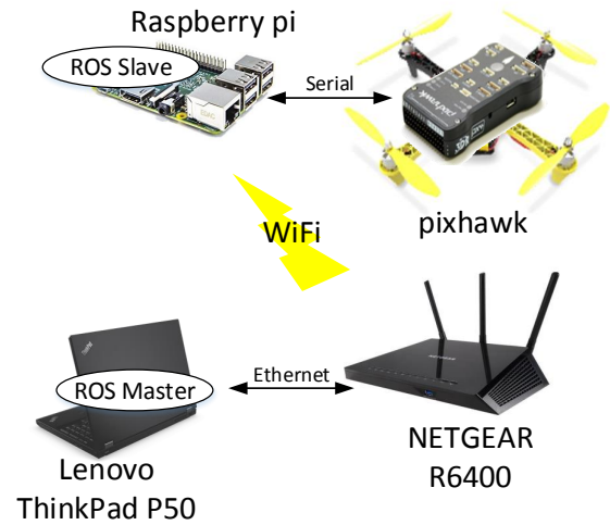
Fig. 1. The Hardware configuration of the hands-on
