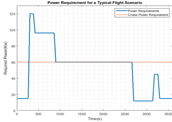
Fig. 4 Power requirement of a typical flight
