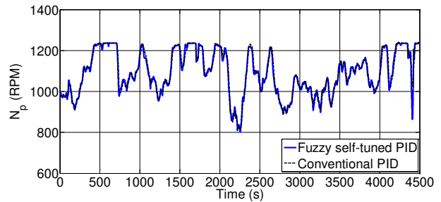
Fig. 21. Variation of pump speed
