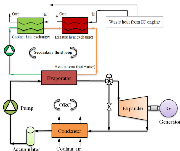
Fig. 2. Dynamic model of ORC-based WHR system.
