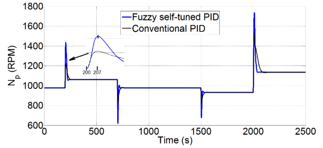
Fig. 14. Variation of pump speed
