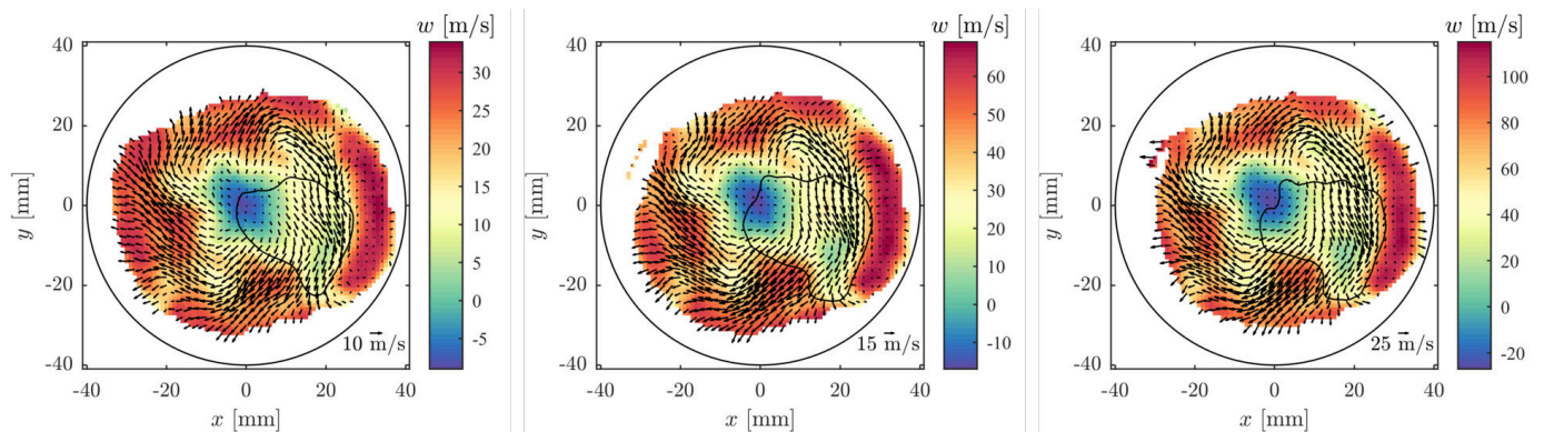
Figure 11. Velocity distribution with the swirl generator installed 20 mm upstream of the ROI. For nominal flow velocities of 30 m/s (left), 60 m/s (center) and 100 m/s (right). The axial velocity is color coded according to the colormap on the right side of each plot. The inplane velocities are overlaid with arrows. The black overlay is the region of the hotstreak.
