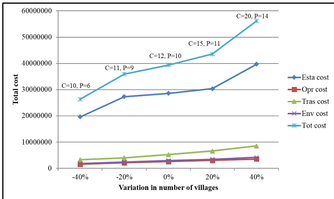
Figure 8 Effect of variation in number of villages on objective function and its components
