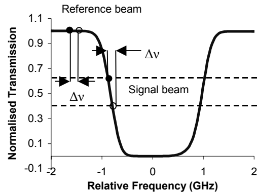
Fig 2. Relative positions of the laser frequency, and the shifted frequency on a typical absorption feature for 2v-PDV (Open circles denote the position of the illumination frequency and closed circles the Doppler shifted frequency.)
